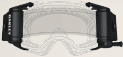
ROLL-OFF ACCESSORY KIT CLEAR (100-258-001) 1 ROLL-OFF CANISTER W/ COVER PLATES 1 ANTI-FRICTION ACCESSORY 2 ROLLS OF FILM 1 MUD GUARD (NOT SHOWN)
